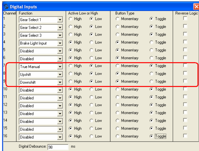
Figure 10 - TCU Digital Input Configuration
