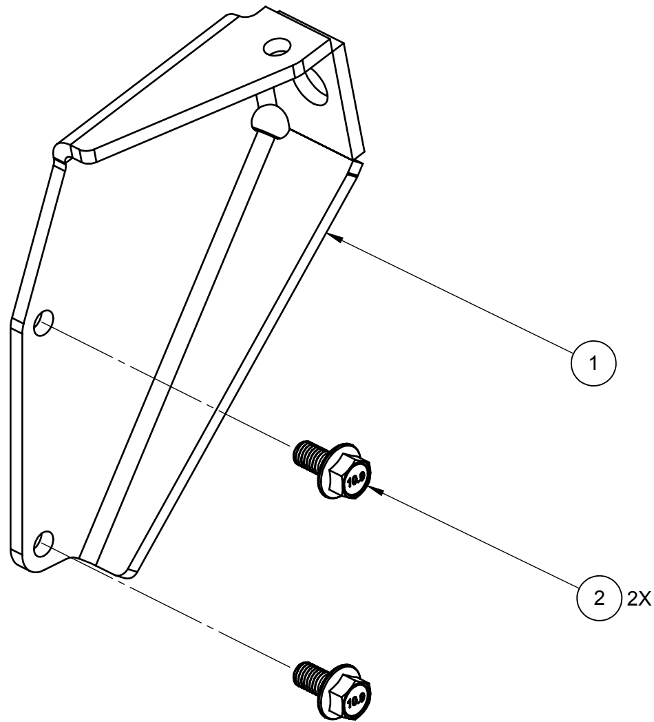
ISO VIEW EXPLODED SCALE: 2:3
