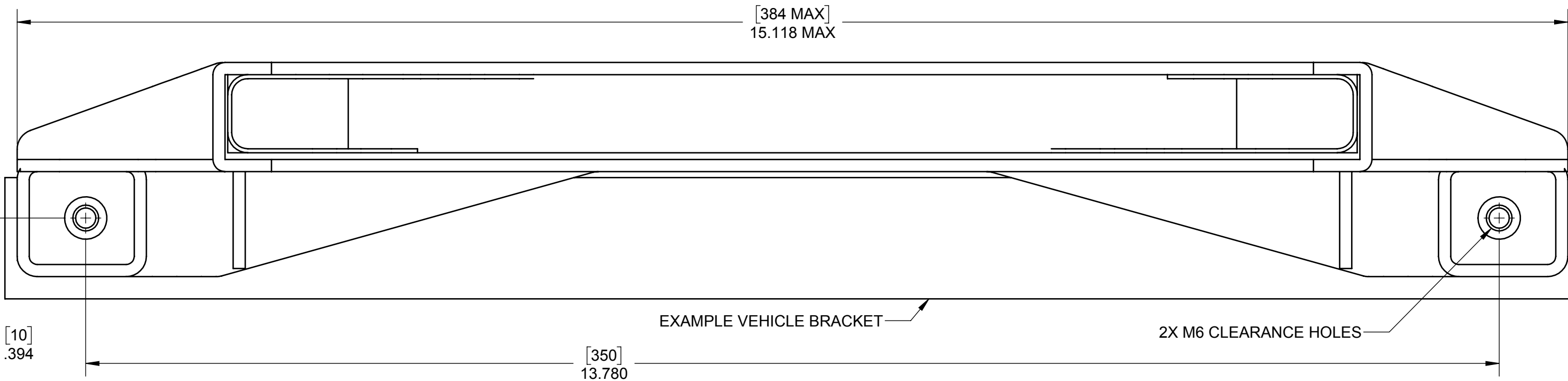
TOP VIEW INSTALLED - TEMPLTE SCALE: 1:1
